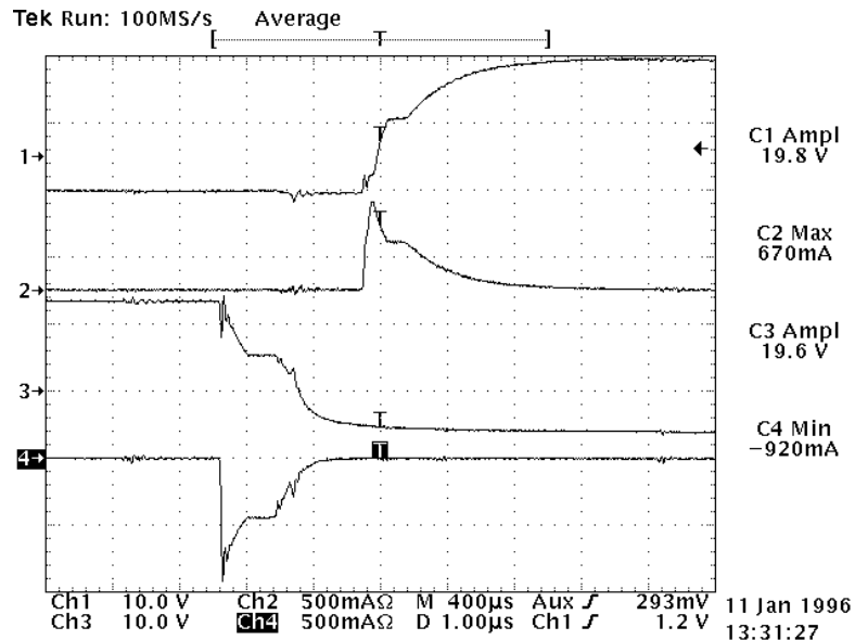
TCP202 – IGBT current and voltage waveforms
